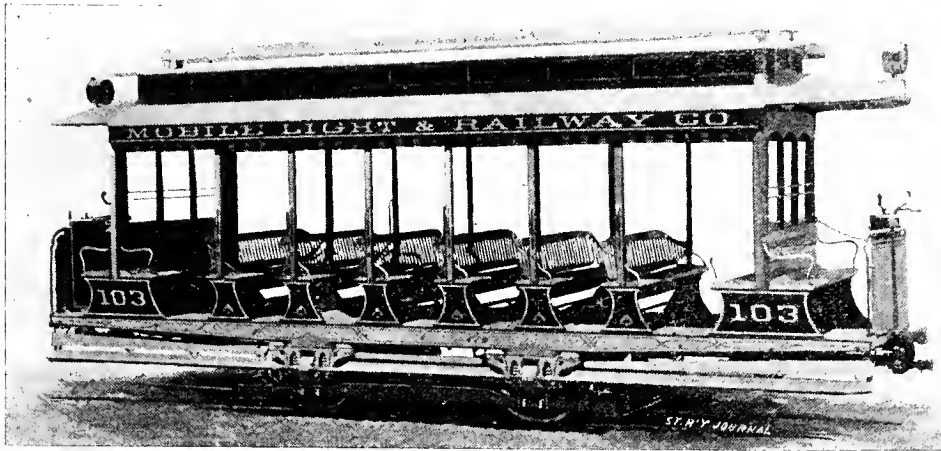
Fig. 5618. OPEN ELECTRIC-MOTOR CAR. THE JOHN STEPHENSON COMPANY. Seating capacity, 50 persons. Ends closed with sashes. Monitor Roof. Tackaberry Truck with Stephenson Super-spring Running Gear.
